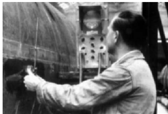
Figure 1.1 A Henry Hughes Mk 2 flaw detector like this was used by Donald in his first experiments.
